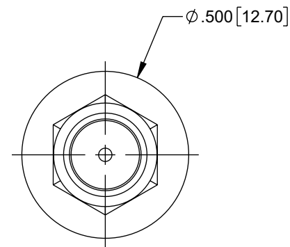
SMA PLUG
